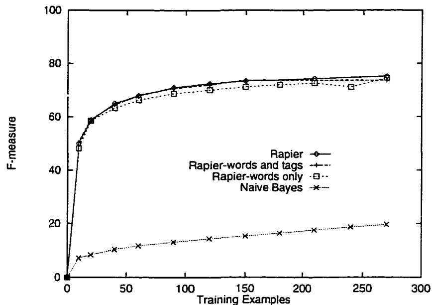
Figure 4.3: F-measure on computer-related job postings
