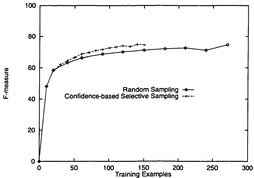
Figure 5.1: Results of selective sampling versus random selection of examples
