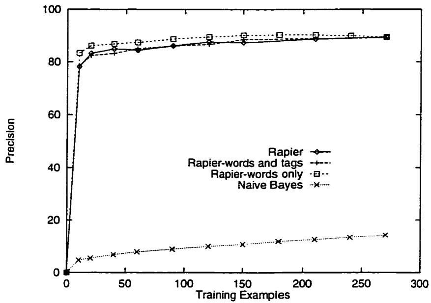
Figure 4.1: Precision on computer-related job postings
