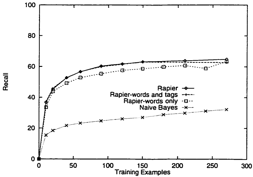
Figure 4.2: Recall on computer-related job postings
